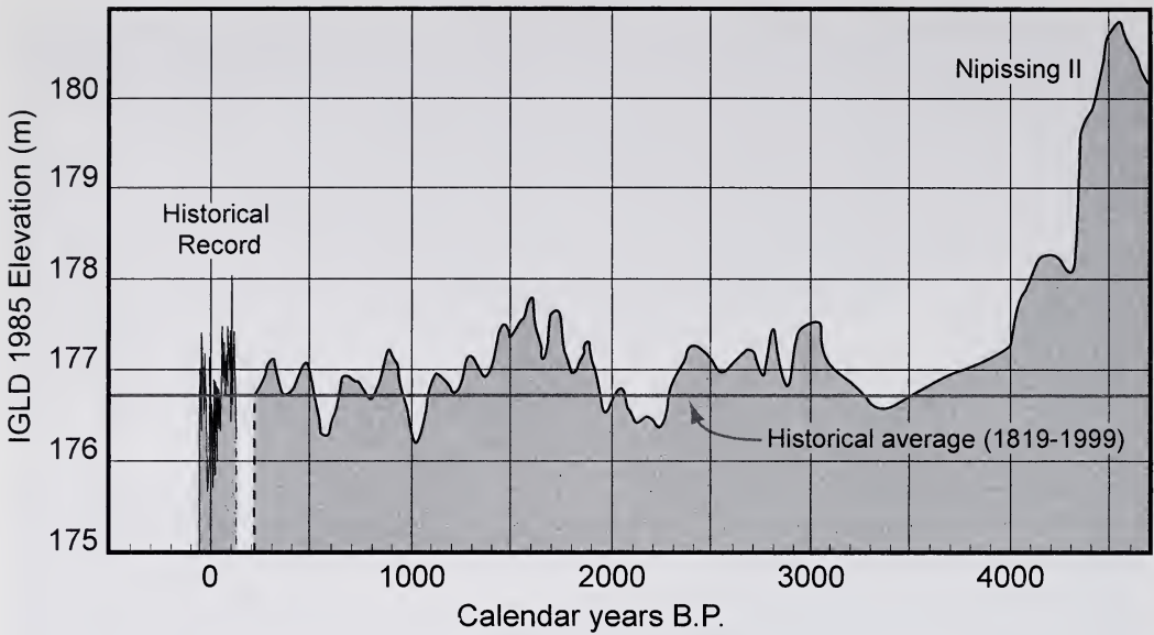
Figure 6.—A Fourier-smoothed lake level curve for Lake Michigan for the last 4700 years. Actual variations in lake level (peaks and troughs) are not shown. This curve combines data sets for around the Lake Michigan basin and illustrates the dramatic drop in lake level from the Nipissing II stage and multiple meter variations in lake level since 4000 ybp when the Toleston Beach was forming. IGLD—International Great Lake Datum. Modified from Baedke & Thompson (2000).
