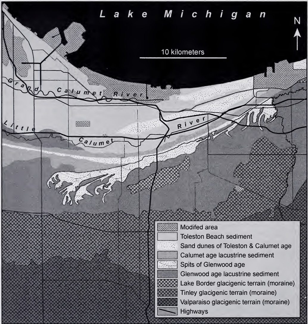
Figure 5.—Generalized Quaternary terrain map for northwest Indiana illustrating the inset relationship of moraines and beaches. As a general rule, the landscape becomes progressively younger from south to north. Modified from Brown et al. (1996).
