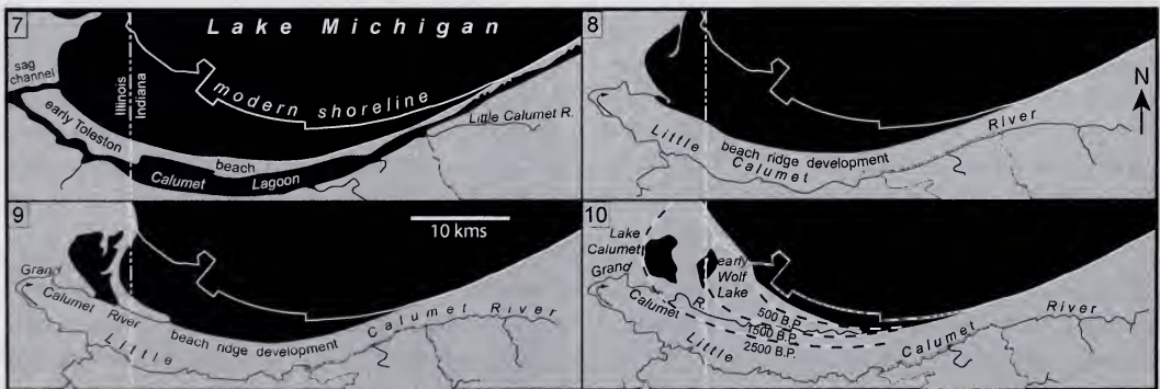
Figure 7-10.—The evolution of the Grand Calumet River was initiated by closing the Sag channel and deflection of the Little Calumet River eastwards by spit and beach ridge growth in the southwest corner of the lake. Figures modified from Chrzastowski & Thompson (1992) and Thompson (1992).
